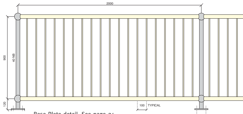
Base Plate detail. See page 24. Jumbo Base Plate Detail. See Page 30.
